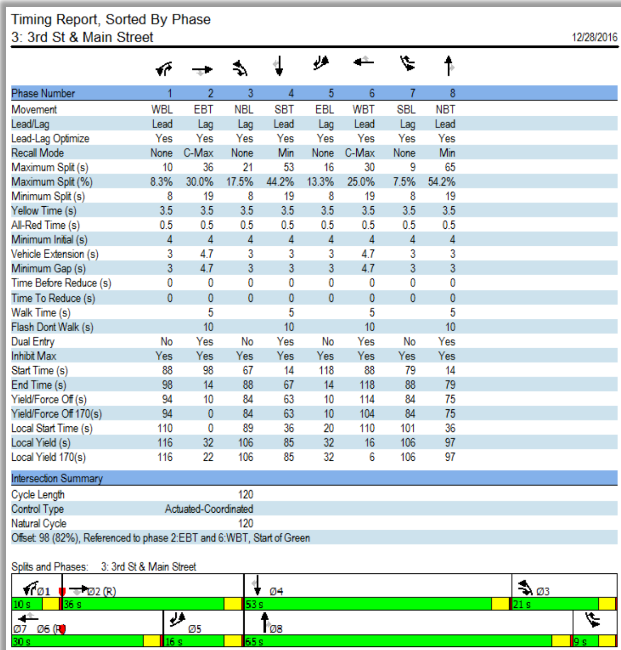
Figure 24-10 Sample Timing Report, Sorted By Phase
