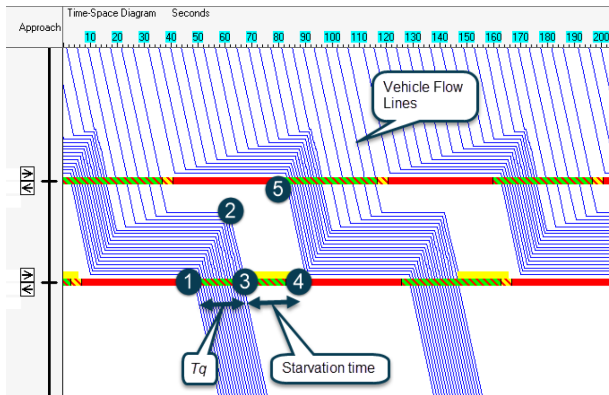
Figure 21-4 Starvation in Time Space view
