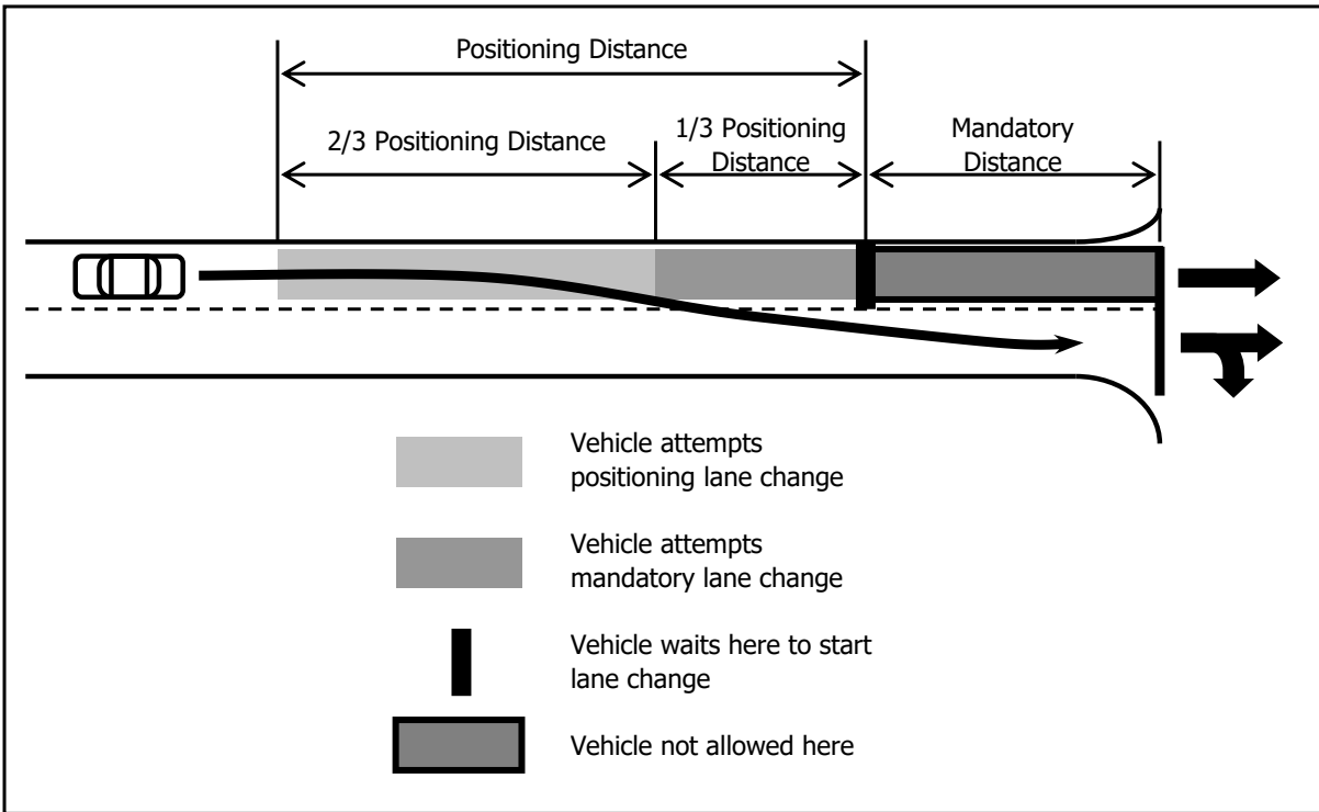
Figure 31-1 Vehicle Turning Right from Left Lane
