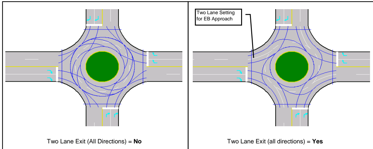
Figure 28-2 Two Lane Exit Coding
