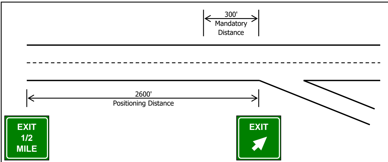
Figure 31-4 Freeway Off-Ramp Lane Change Distances
