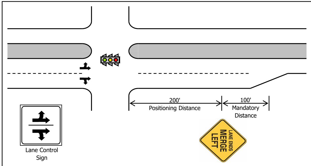
Figure 31-7 Lane Drop after Signal
