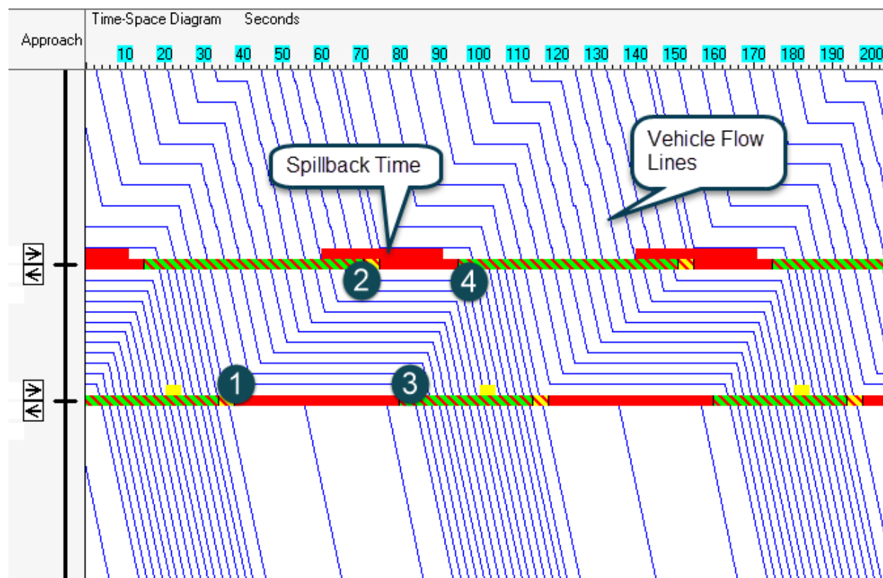
Figure 21-7 Spillback in Time Space view
