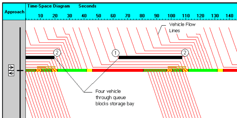
Figure 21-8 Storage Blocking in Time Space view (Through Traffic)
