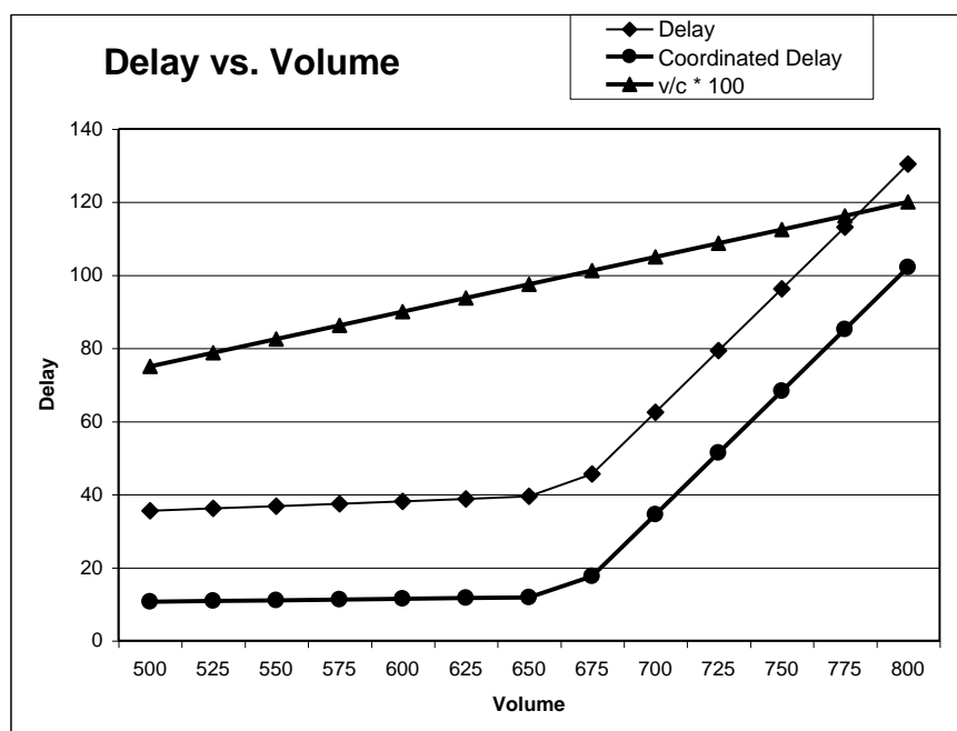
Figure 21-16 Delay vs. Volume
