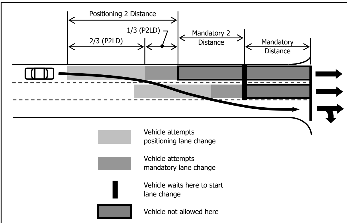
Figure 31-2 Vehicle Turning Right Making Two Lane Changes
