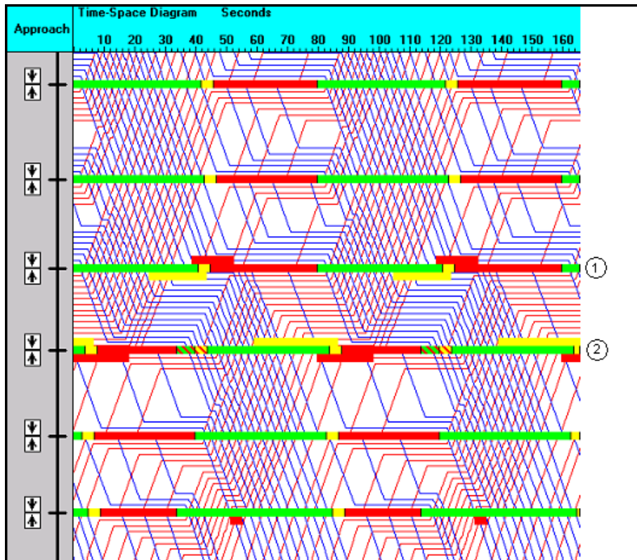
Figure 21-12 Flow Line Diagram
