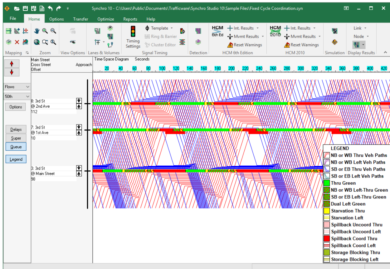
Figure 19-1 Time-Space Diagram
