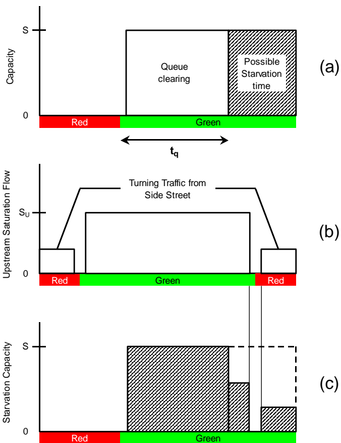
Figure 21-5 Starvation Capacity Reduction
