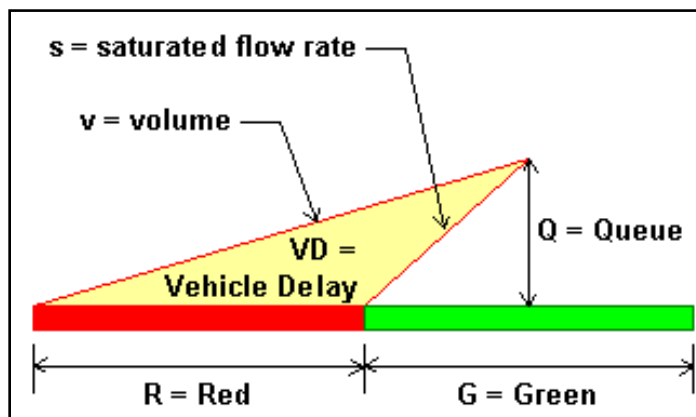
Figure 21-14 Arrival Departure Graph
