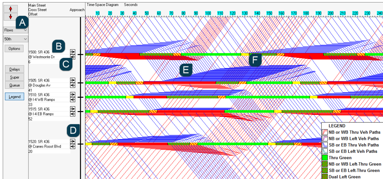
Figure 19-2 Parts of a Time-Space Diagram
