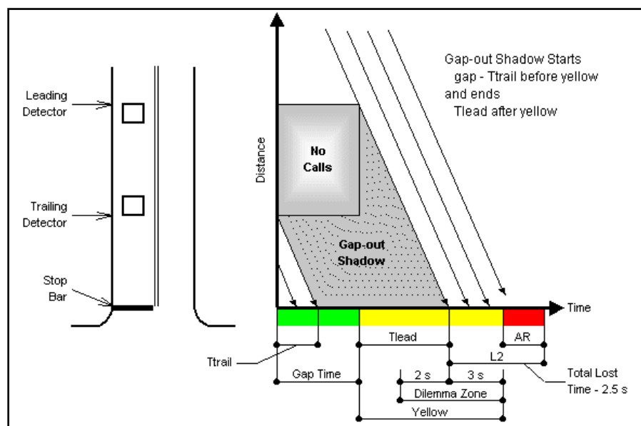
Figure 21-15 Dilemma Zone Gap Out Shadow
