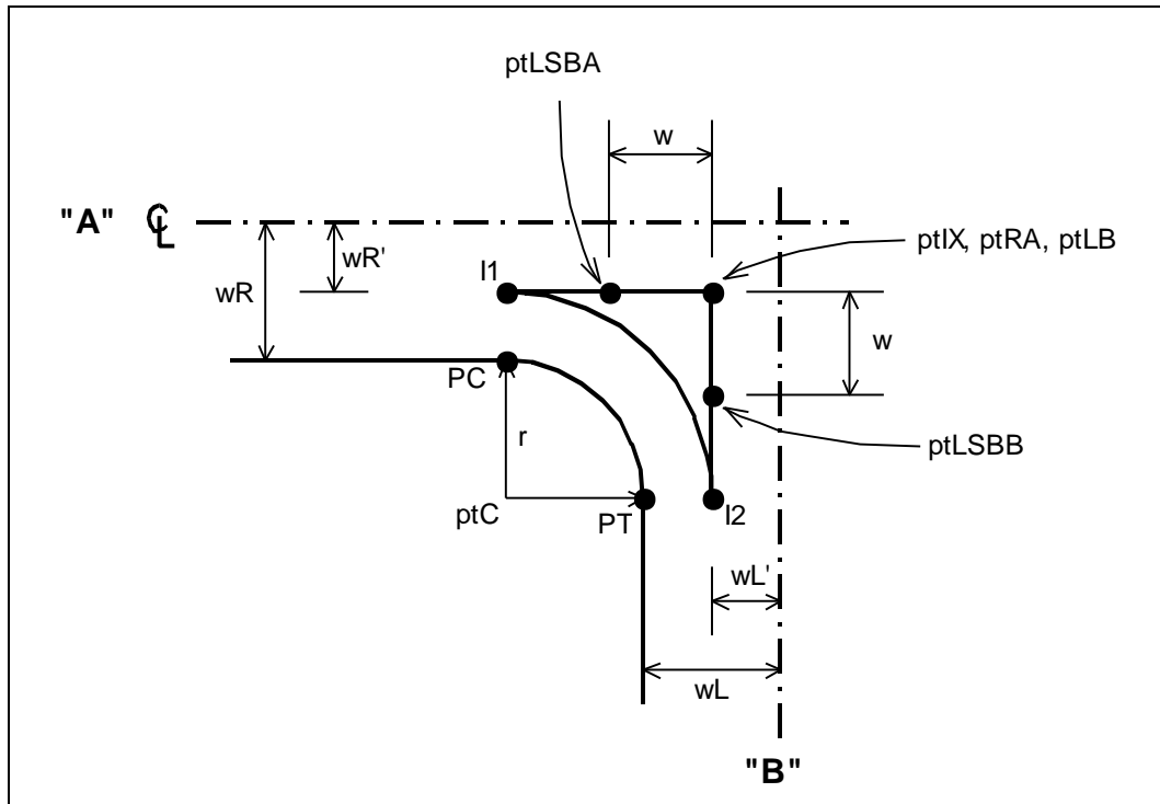
Figure 31-14 Right Turn Island
