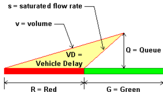
Figure 21-1 Vehicles Queued at Red light
