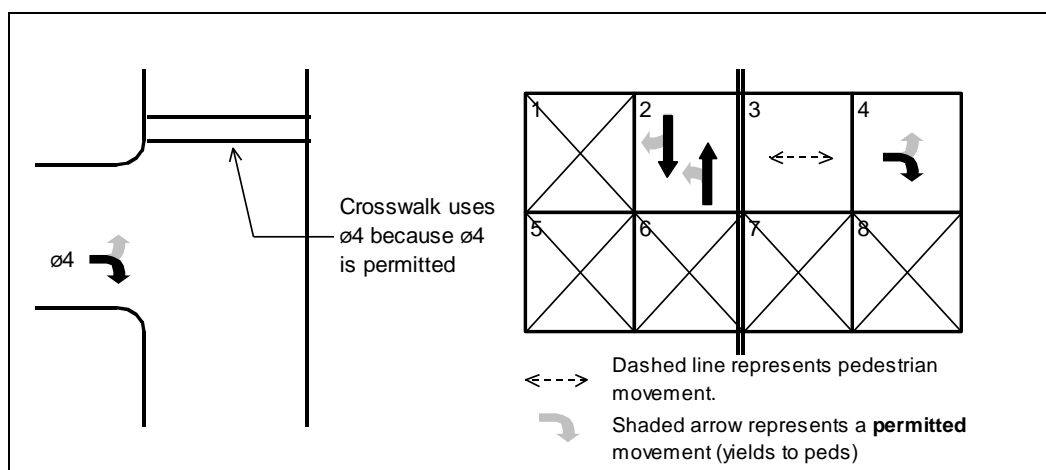
Figure 28-7 Pedestrian Phase with Permitted Left Turn Phase
