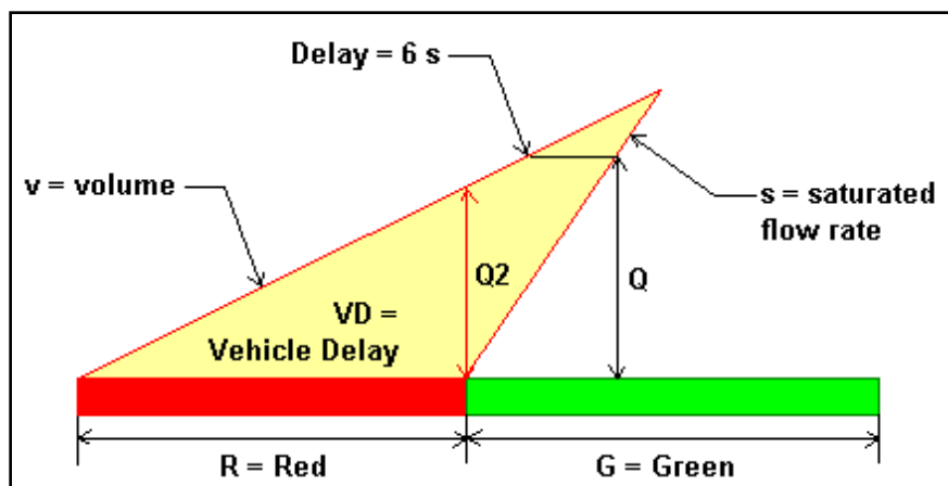
Figure 21-13 Arrival Departure Graph
