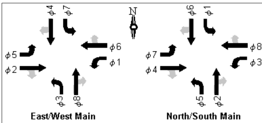
Figure 11-9 Phase Template
