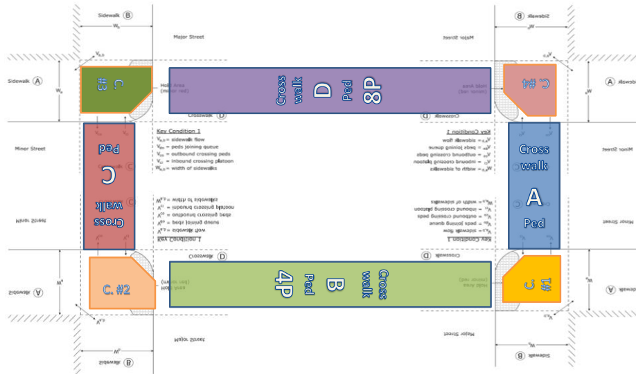
Figure 18-5 HCM 2010 Pedestrian Mode Crossing Diagram
