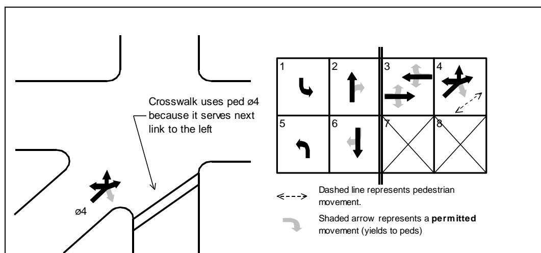
Figure 28-5 Pedestrian Phase at a Five-Leg Intersection
