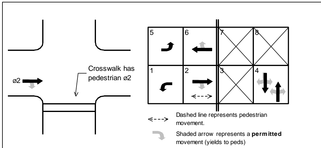
Figure 28-3 Pedestrian Phase Associated with Through Phase
