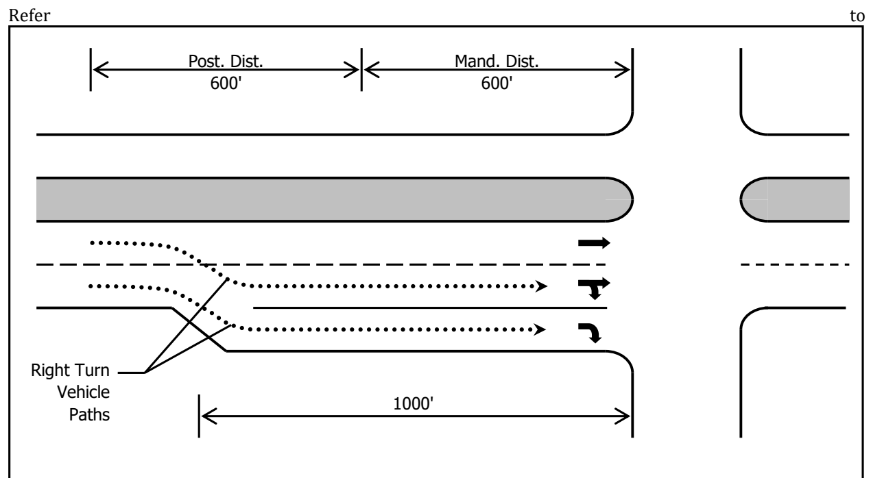
Figure 31-9. There is a long turning bay for right turns and dual right lanes at the signal. The right turn movement has a lot of volume. The goal is to allow some right turning vehicles to use the left lane and merge right after the start of the storage bay.
