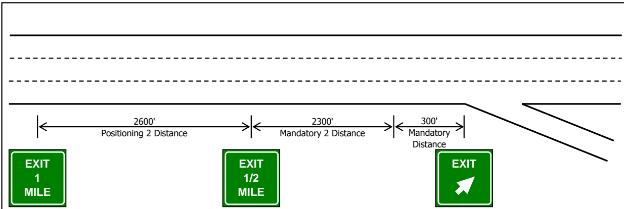
Figure 31-6 Freeway Off-Ramp Lane Change Distances (Three-Lane Freeway)
