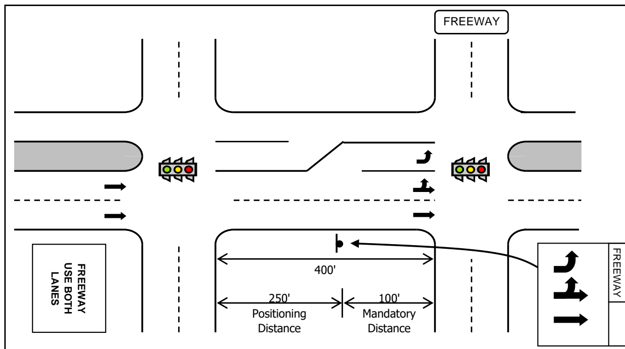
Figure 31-10 Lane Change through Multiple Intersections
