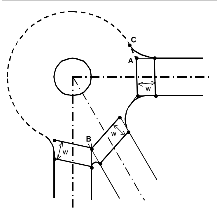
Figure 31-15 Roundabout
