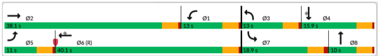
Figure 11-5 Splits and Phasing Diagram Example
