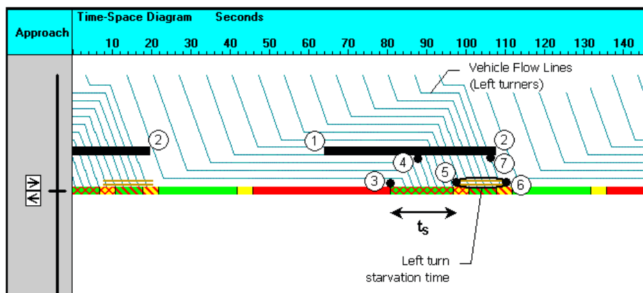
Figure 21-9 Storage Blocking in Time Space view (Left Turn Traffic)
