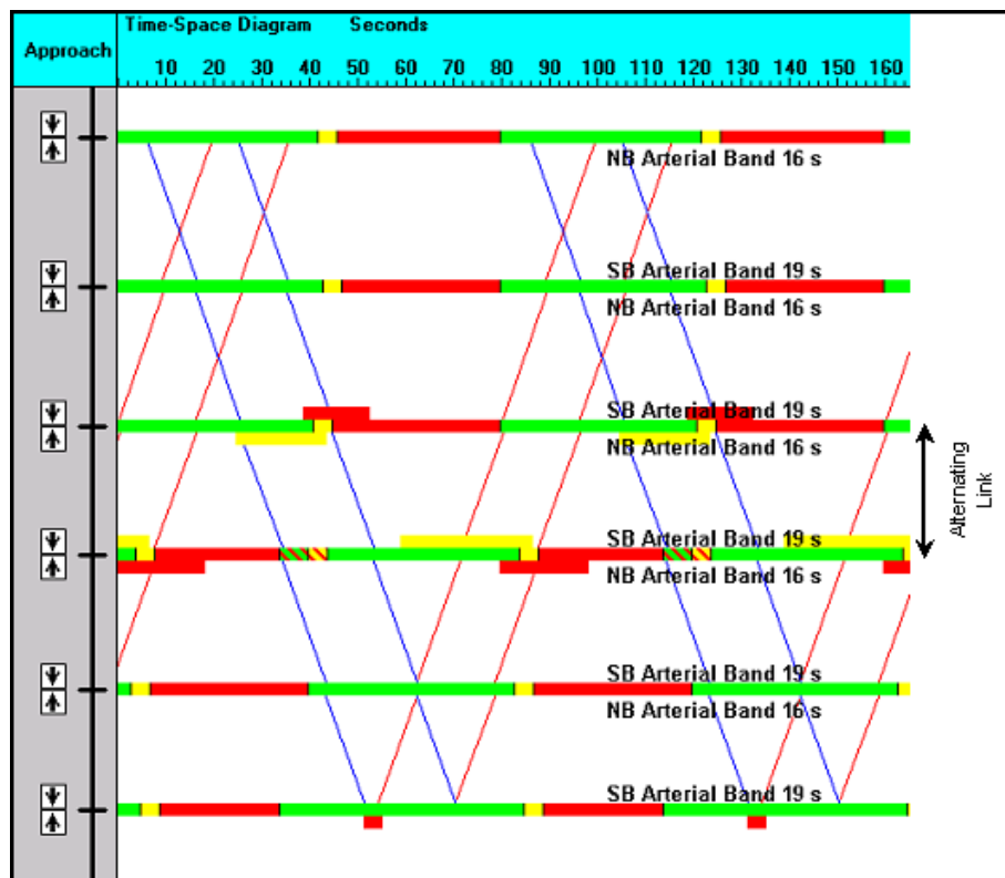
Figure 21-11 Two-Way Bandwidth
