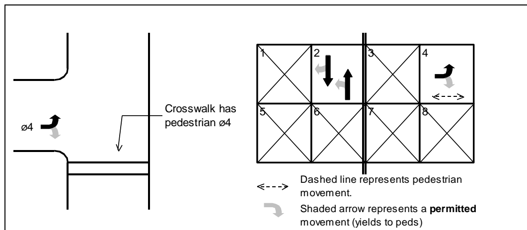
Figure 28-4 Pedestrian Phase Associated with Left Phase
