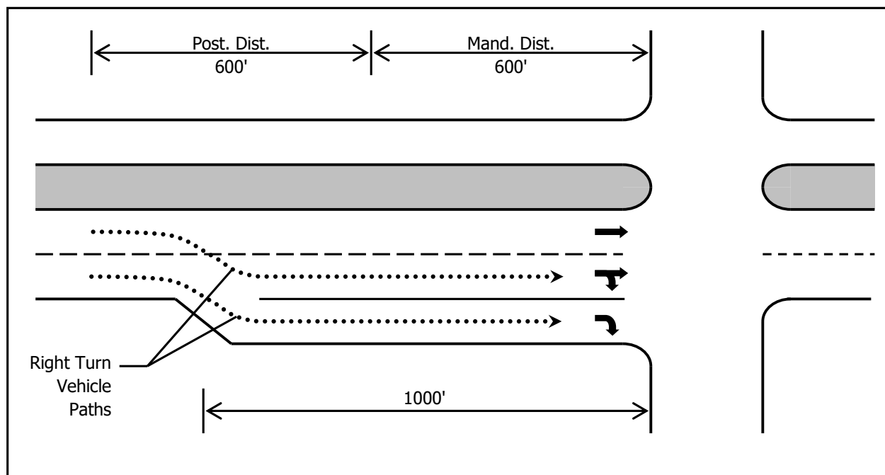
Figure 31-9 Long Turning Bay Example
