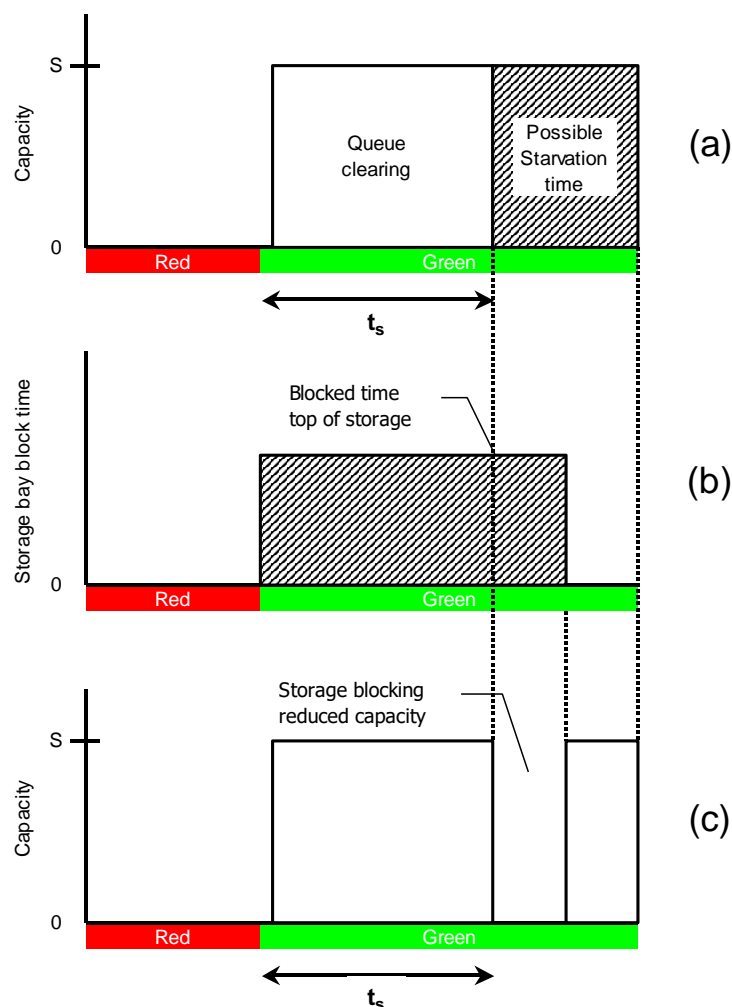
Figure 21-10 Storage Blocking Capacity Reduction
