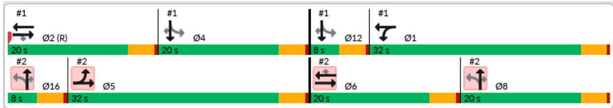
Figure 11-6 Group Control Example
